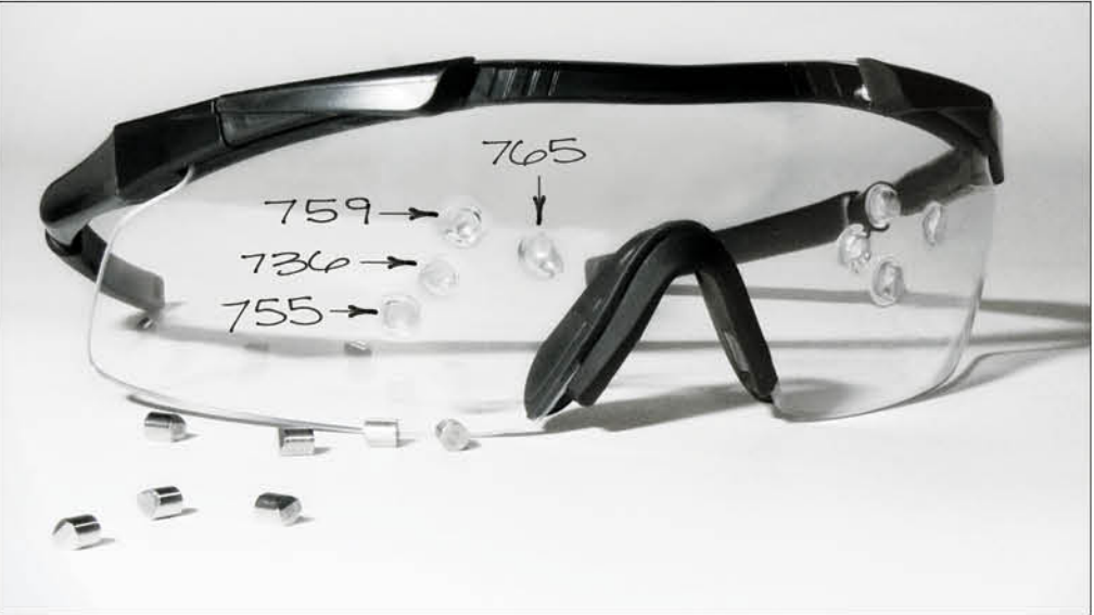
IMPACTED BY A 0.15 CALIBER, 5.8 GRAIN, T37 SHAPED PROJECTILE.
